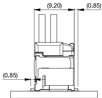
嵌合図 MATED CONNECTORS
